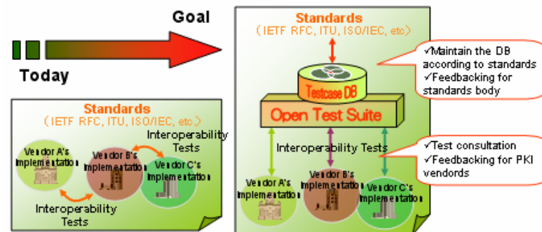
The concept of the open test suite
